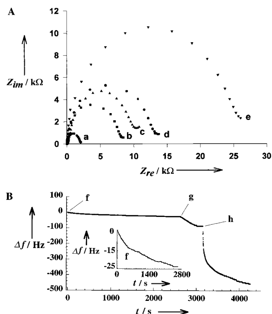
Figure 5. A) Faradaic impedance spectra (Nyquist plots) upon the amplified sensing of VSV RNA: a) the 5 -functionalized electrode; b) after hybridization with the VSV RNA, 1 \times 10^{-12} \text{ M} , in a solution consisting of 40 mM PIPES, 1 mM EDTA, 400 mM NaCl, 80% formamide, pH 7.5; c) after the reverse transcription for 45 min ( 80 \text{ U mL}^{-1} ) in the presence of dGTP, dATP, dTTP, dCTP, and biotinylated dCTP (1:1:2/3:1/3 base concentration 1 mM) in a solution consisting of 50 mM Tris buffer, 40 mM KCl, 8 mM \text{MgCl}_2 , pH 8.3 at room temperature; d) after the association of the avidin–alkaline-phosphatase conjugate, bulk concentration 1 mM; e) after the biocatalyzed precipitation of 3 for 20 min in the presence of 2 ( 2 \times 10^{-3} \text{ M} ) in Tris buffer pH 7.5. B) Time-dependent frequency changes of an Au-quartz crystal upon the analysis of the VSV RNA ( 1 \times 10^{-12} \text{ M} ); f) frequency changes as a result of the replication of the bound RNA in the presence of reverse transcriptase and dGTP, dATP, dTTP, dCTP, and biotinylated-dCTP; g) upon the association of the avidin–alkaline-phosphatase conjugate; h) Upon the biocatalyzed precipitation of 3 . The conditions for the polymerization and biocatalyzed precipitation of 3 are detailed in Figure 5A. Inset: Magnification of curve f.
